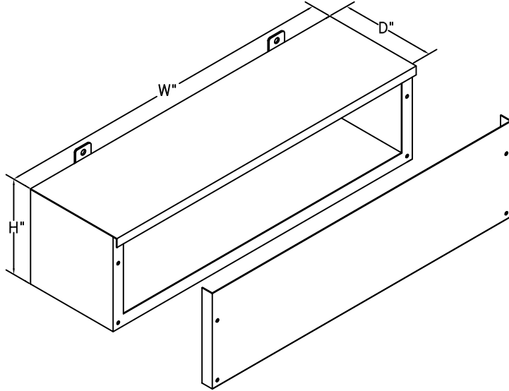
WALL MOUNTED
